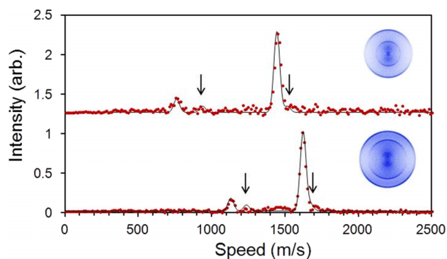
FIG. 2. S branch CO ion images with their corresponding speed distributions and simulations at 213.478 nm on the top and 213.615 nm on the bottom. The inner rings originate from v=1 CO while the outer rings originate from v=0 CO. The top panel corresponds to j=63 for the outer ring and j=67 for the inner ring and the bottom panel corresponds to j=58 for the outer ring and j=61 for the inner ring. Filled circles are for the experimental speed distribution, while the solid lines show the simulated speed distribution. Minor contributions of CO products originating from vibrationally excited parent OCS are also shown and their locations are marked by arrows.
