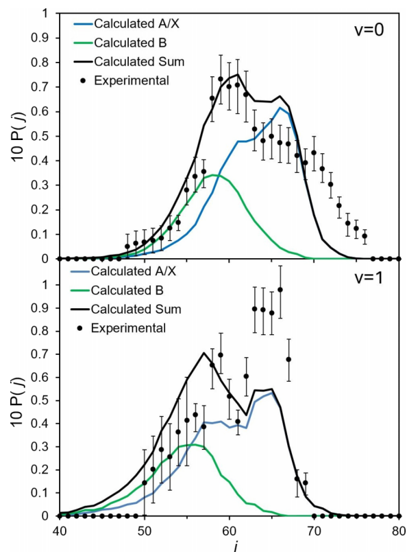
FIG. 3. CO rotational distributions associated with v=0 (upper panel) and v=1 (lower panel). In both panels, the experimental data are shown with filled circles and compared to the results of classical trajectory calculations (solid lines). The computed contributions from the A/X and B pathways are shown with blue and green lines, respectively, for both v=0 and v=1 CO products. The rotational populations have been normalized and scaled.
