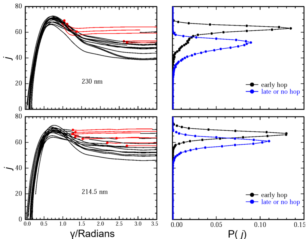
FIG. 6. Left panels: Individual trajectories begun on the A state and propagated with the possibility of surface hopping to X, plotted in (\gamma, j) coordinates. Portions of each trajectory on the A state are in black and on the X state are in red, with the first hop from A to X indicated with a red dot. Right panels: rotational distributions from the entire trajectory set (50 000 trajectories at each wavelength), divided into two groups that did or did not hop from A to X while \gamma < 1.7 .
