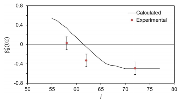
FIG. 8. The \beta_0^2(02) bipolar moment for different rotational states. The experimental values are represented by the filled circles at j = 58, 62 , and 72 . The calculation is represented by the black line.
