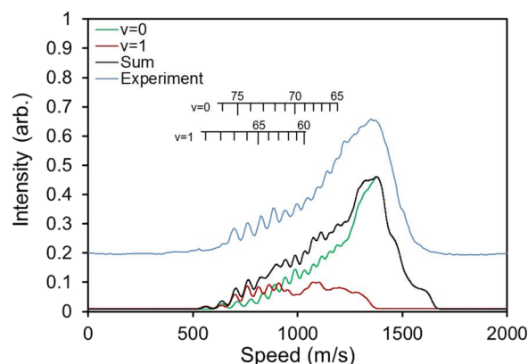
FIG. 5. The speed distribution derived from the DC sliced S(^1D_2) image shown in Figure 4. The simulation consists of two components based on the rotational distributions from the REMPI spectrum, v=0 in green and v=1 in red. The v=1 population of 21% is shown which was obtained from the REMPI spectrum.
