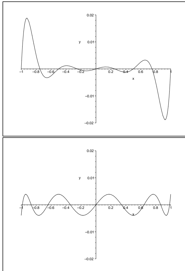
Figure 1: Degree 9 equispaced and Chebyshev polynomials. The equispaced polynomial is scaled to have all its zeros in [-1, 1] ; the Chebyshev polynomial is scaled to be monic.
